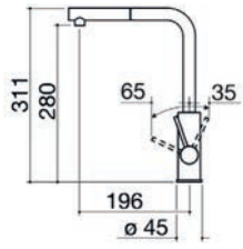
Barazza OFFICINA SHOWER 316
