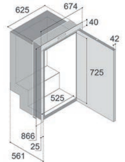
Vitrifrigo C180 stainless steel door refrigerator
