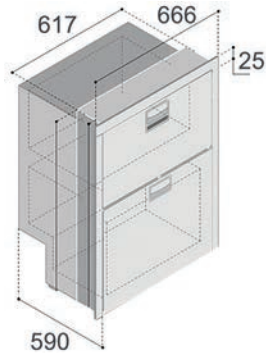
Vitrifrigo DRW180a stainless steel refrigerator and/or freezer
